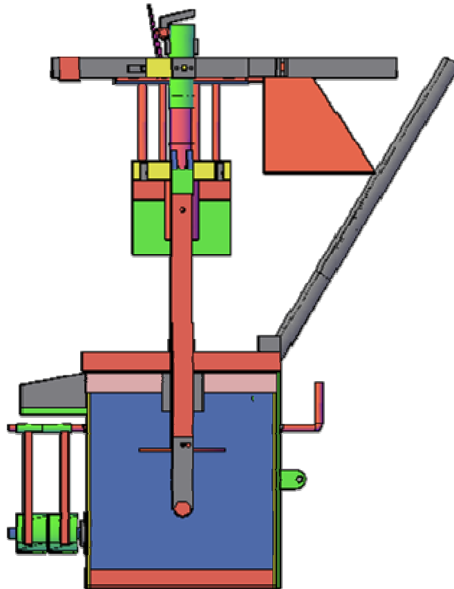
Fig. 3. Side view of the double mould vibration compactor block moulding machine
