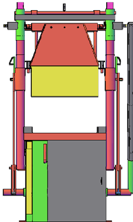
Fig. 5. Front view of the double mould vibration compactor block moulding machine
