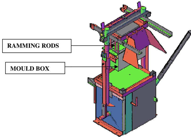
Fig. 4. 3D isometric view of the double mould vibration compactor block moulding machine
