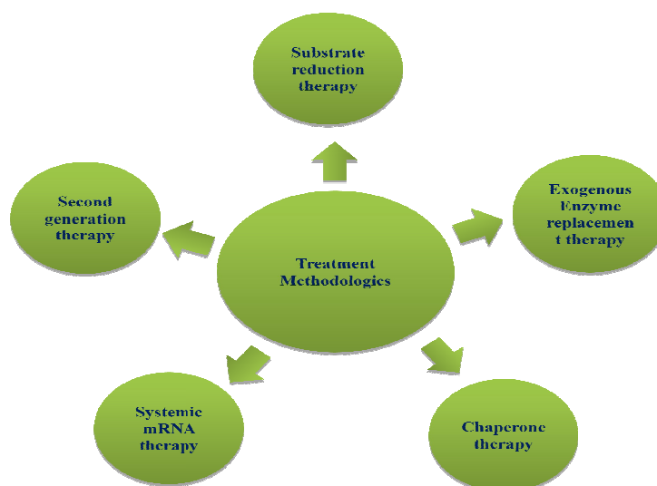
Fig. 5. Methodologies of fabry treatment
