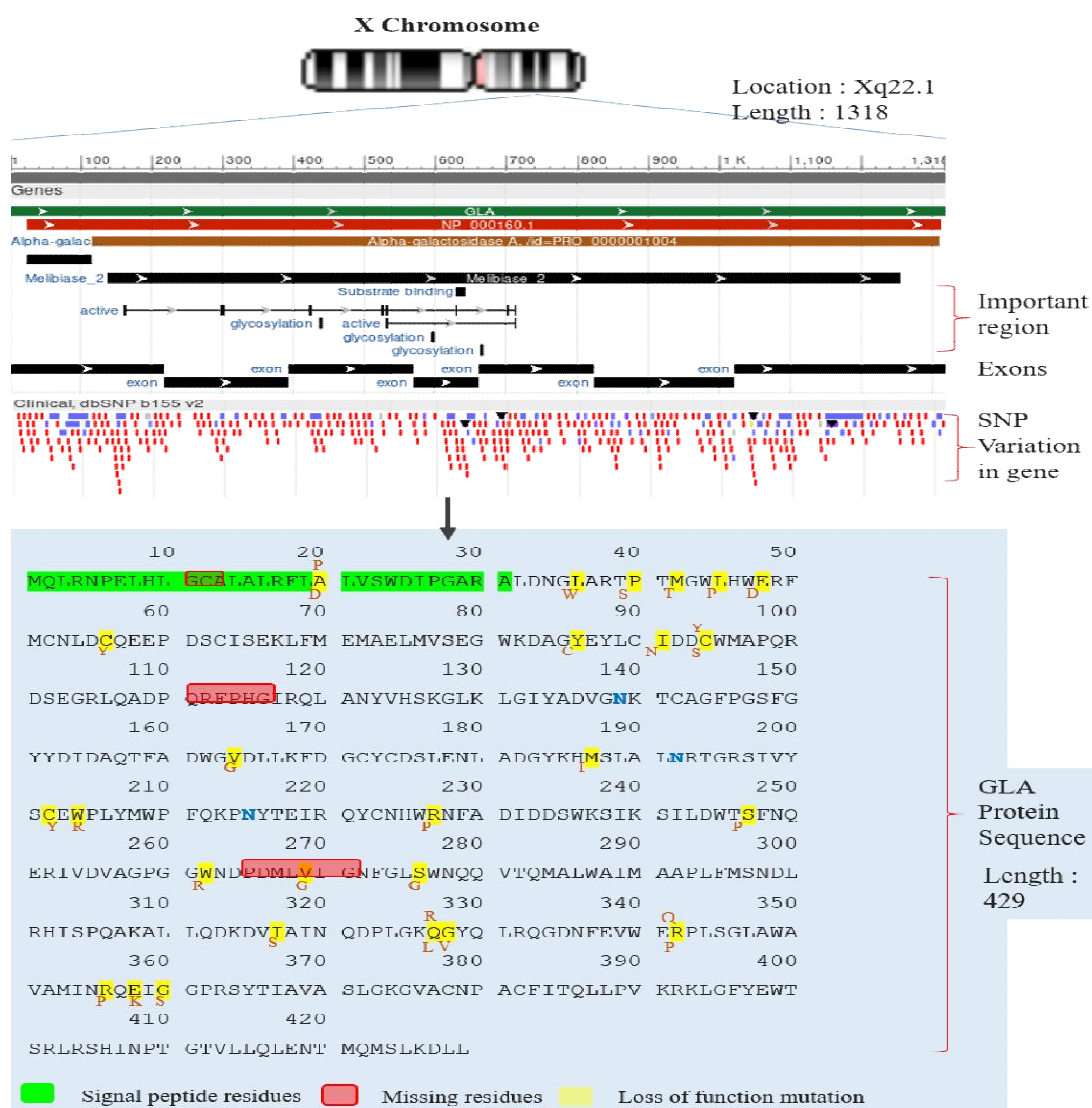
Fig. 2. GLA: Gene to protein sequence and its variations
