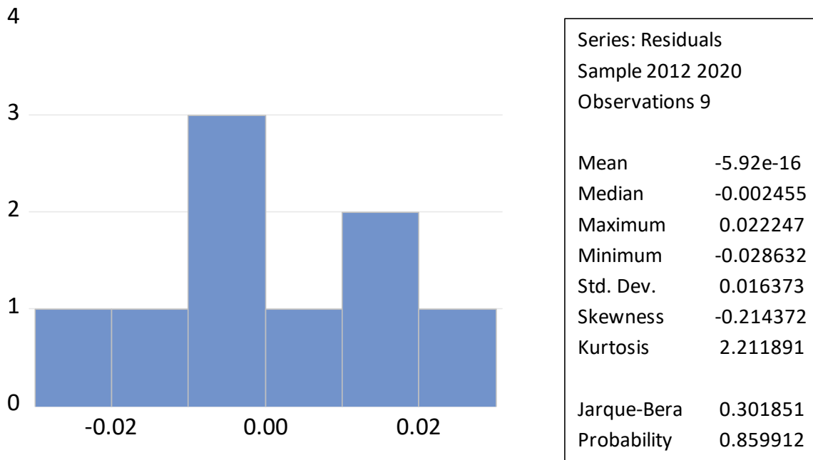
Fig. 2. Normality test
