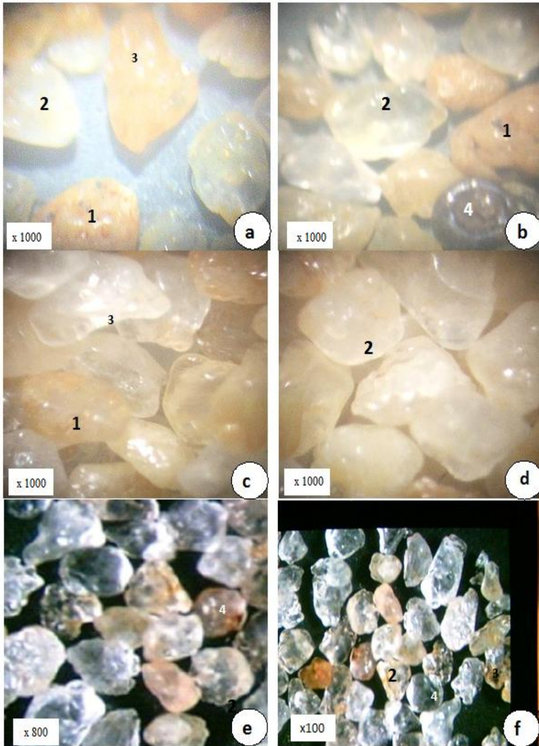
Fig. 2. Morphoscopy of quartz grains in some areas of study
