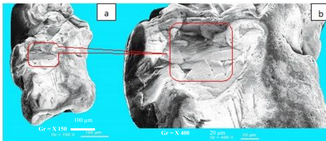
Fig. 5. Traces of shock and some internal figures on a grain of quartz of Grand-Bassam (data [15])
