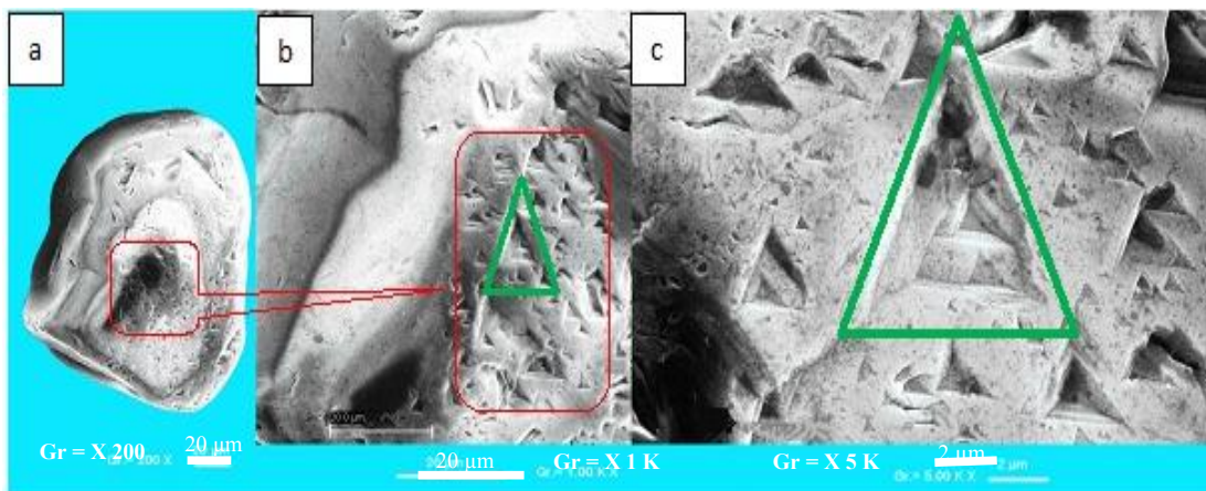
Fig. 8. Traces of dissolution and triangular figures on the beaches west of the mouth of the Aby lagoon in Assinie (data [15])
