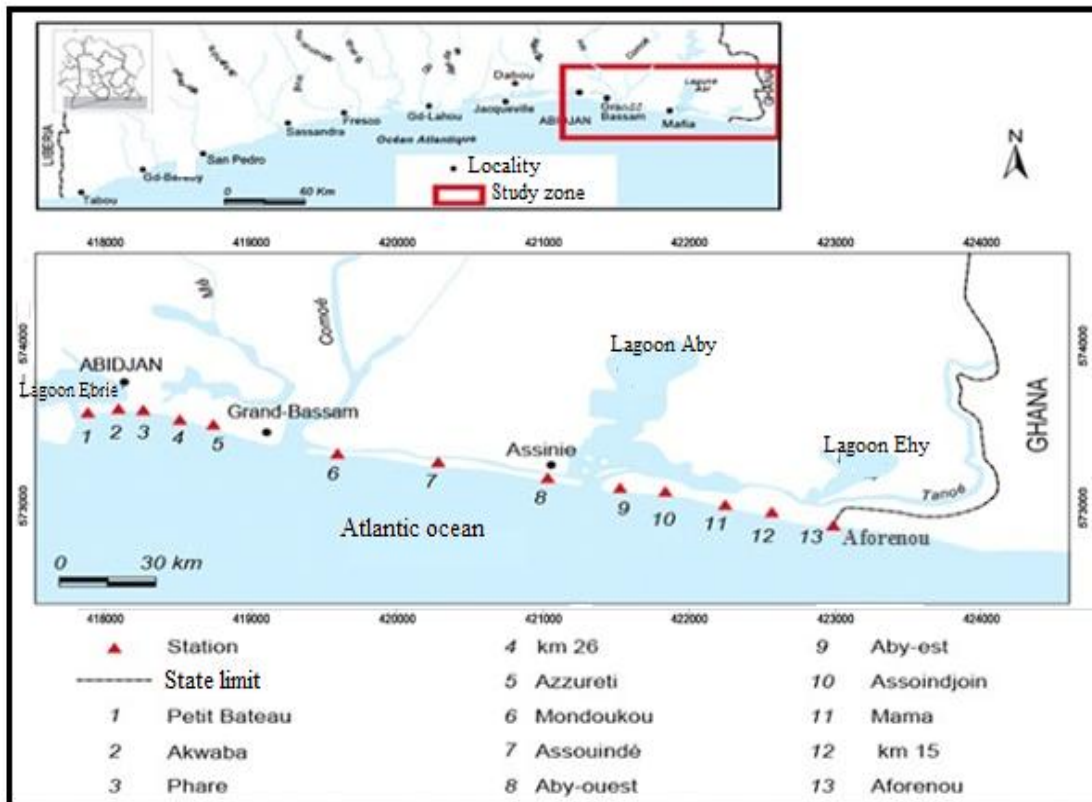
Fig. 1. Study area and presentation of sampling points [15]
