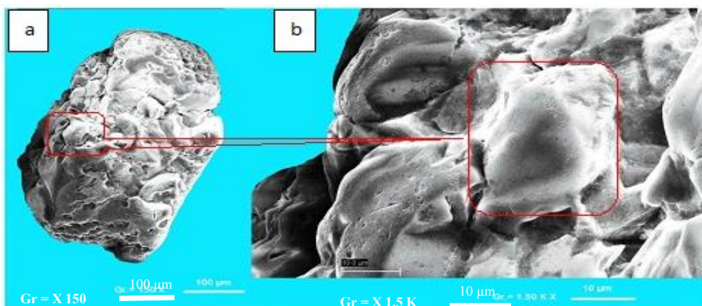
Fig. 10. Dissolution of the entire surface of the quartz grain generating rounded micro-reliefs to the west of the mouth of the Aby lagoon in Assinie (data [15])
