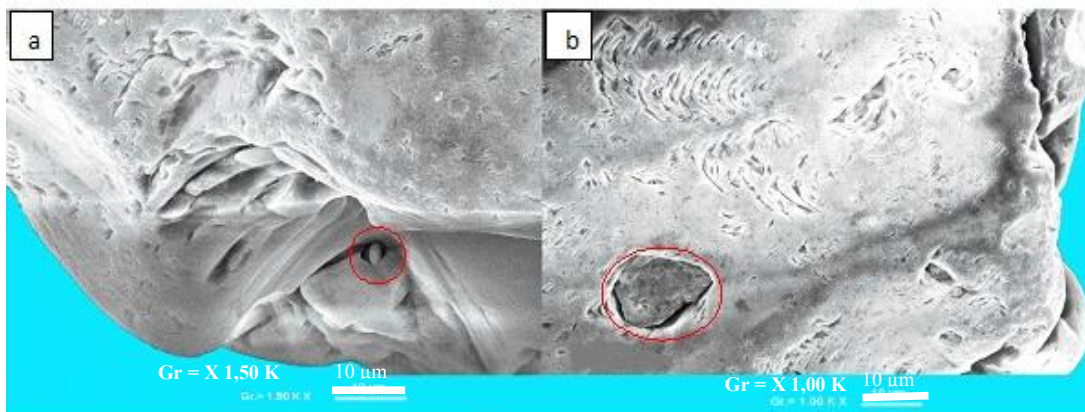
Fig. 13. Traces of shocks and inclusions on the surface of the quartz grains of the beaches east of the Aby lagoon in Assinie (data [15])
