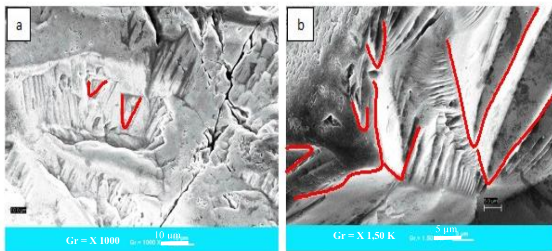
Fig. 12. Appearance of the "V" figures and pressure traces (b) on quartz from the beaches east of the mouth of the Aby lagoon in Assinie (data [15])
