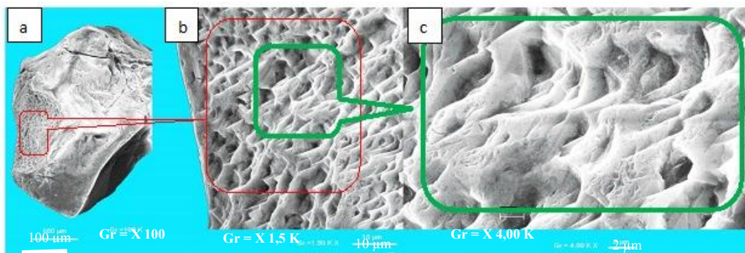
Fig. 11. Chemical dissolution appearing on the tops of a quartz grain from the beaches east of the mouth of the Aby lagoon in Assinie (data [15])
