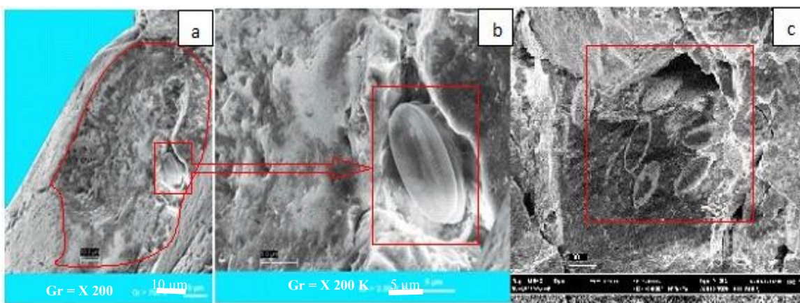
Fig. 4. Diatom housed in the shock traces of some quartz grains (data [15])
