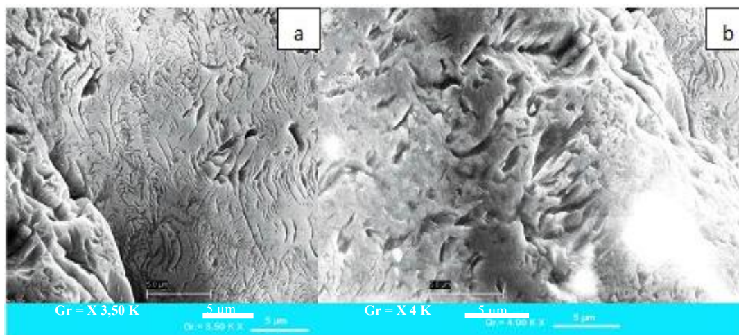
Fig. 6. Marks of superficial chemical dissolution on a Grand-Bassam quartz grain (data [15])
