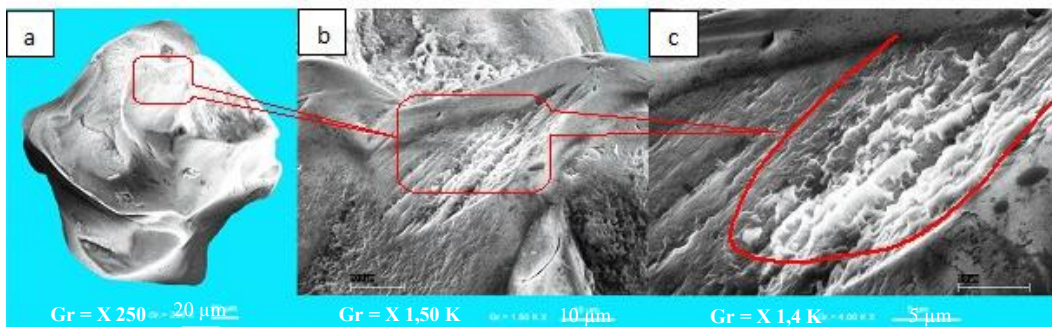
Fig. 9. Chemical dissolution of the surface of a quartz grain from the beaches west of the mouth of the Aby Lagoon in Assinie (data [15])
