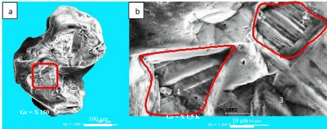
Fig. 16. Sand grain with many traces of shocks with dissolution figures in Aforenou (Ghana) (1, 2 and 3 = Parallel lines containing disaggregated particles; data [15])
