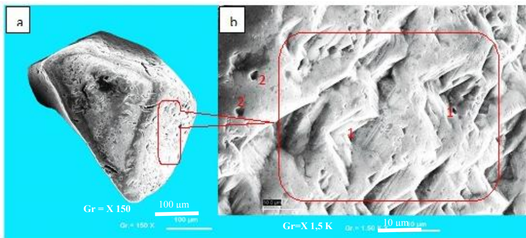
Fig. 14. Important corrosion of the quartz grain in the form of cavities in which are visible parallel lines arranged in stairs at Aforenou (Ghana) (data [15]) (1-Cavities in stairs whose vertices form angles; 2-Primary points of corrosion)
