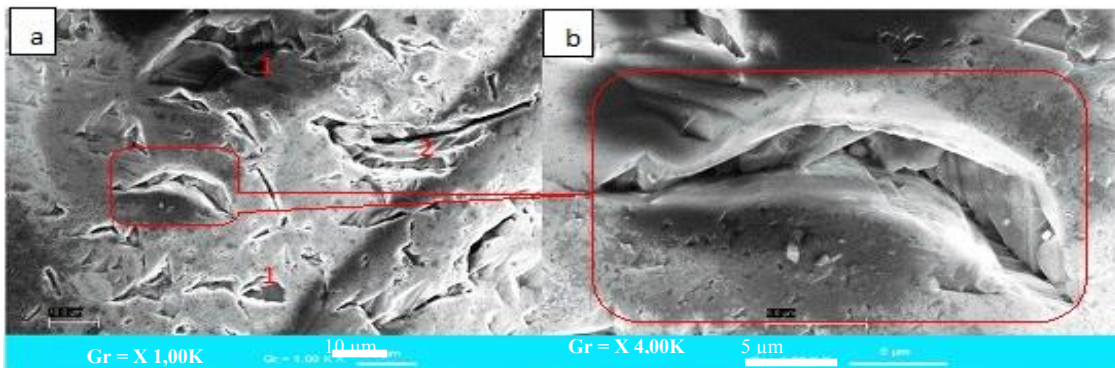
Fig. 15. Numerous nail strokes appear in Aforenou (Ghana) (1 and 2 = traces of old shocks and blunted by fluvial wear, data [15])
