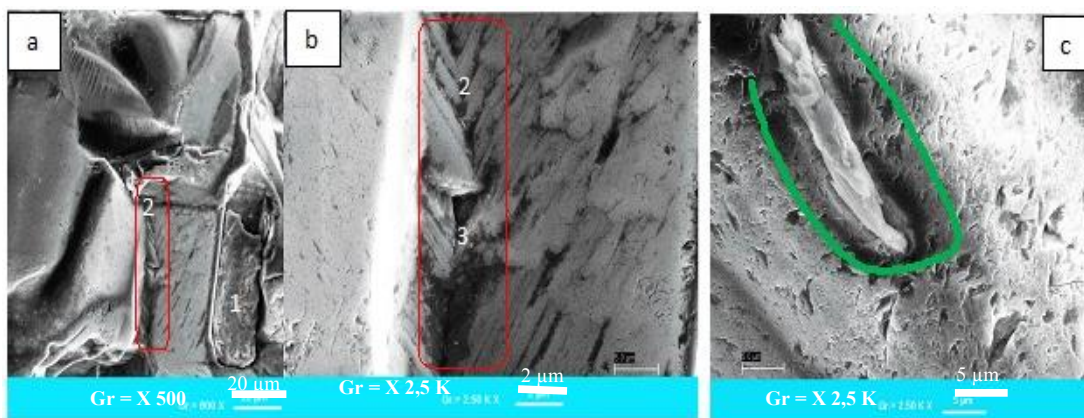
Fig. 7. Inclusions on the surface of certain quartz grains of the beaches of Grand-Bassam (data [15]) (a) magmatic, (b) glassy, (c) cavities
