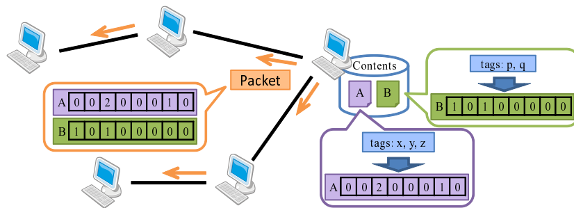
Figure 7: SBF distribution.
