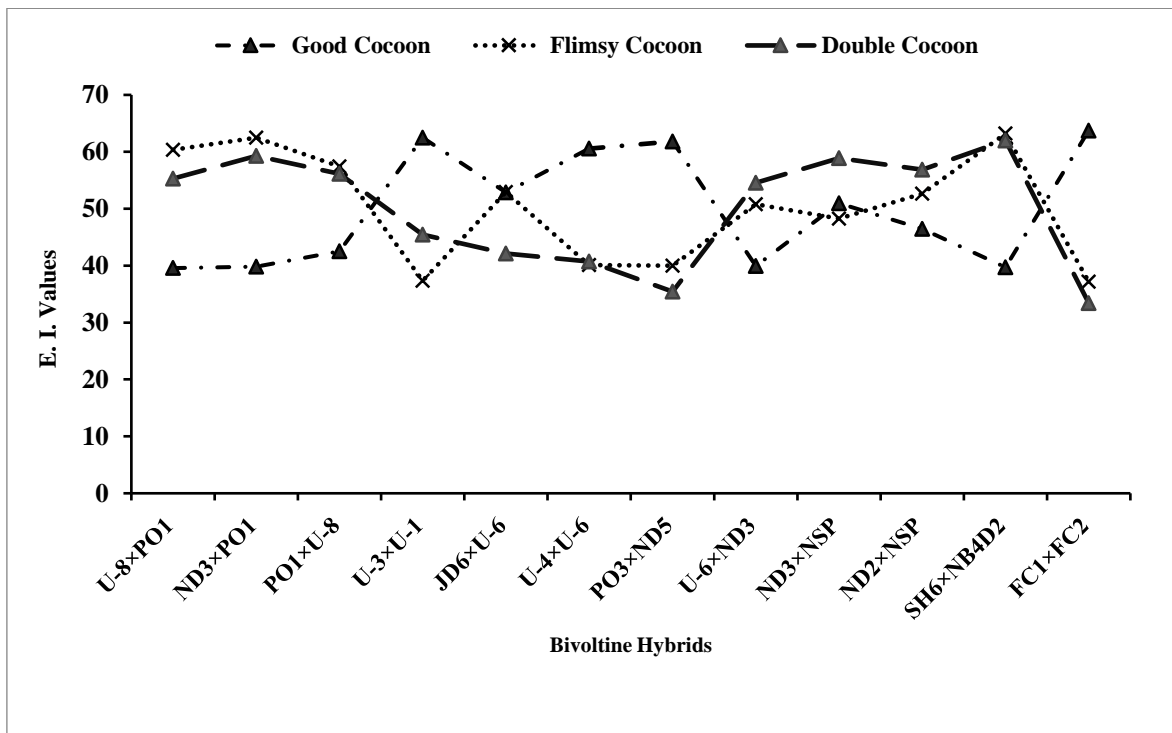
Fig. 4. Evaluation Index values of silkworm bivoltine hybrids for different cocoon traits
