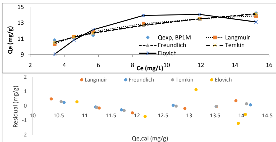
Fig. 6. Non-linear isotherm and residual plot for two parameters in the case of BP1M
