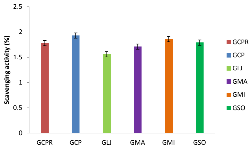
Fig. 4. Scavenging activity of local cheese produced from goat milk using different biocoagulants
