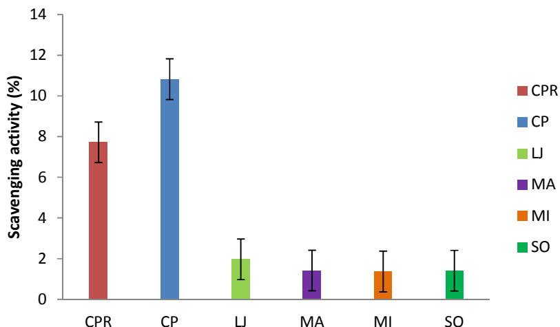
Fig. 3. Scavenging activity of bio-coagulants used in the production of local cheese on DPPH free radical
