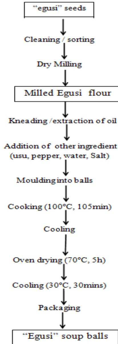
Fig. 1. Flow chart for the production of “egusi” ( Citrullus vulgaris ) Soup Ball
